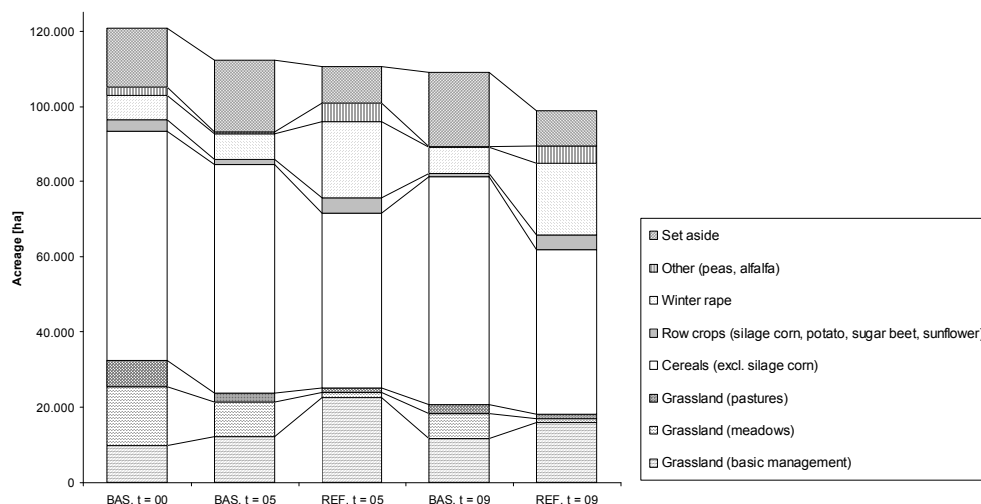
Figure 1. Land use changes at regional level by scenario; t=00 , 05 and 09.
