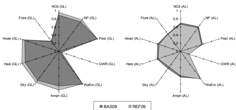
Figure 2. Aggregated IGA values at the regional level for aeable land (AL) and grassland (GL) by indicator and scenario.
